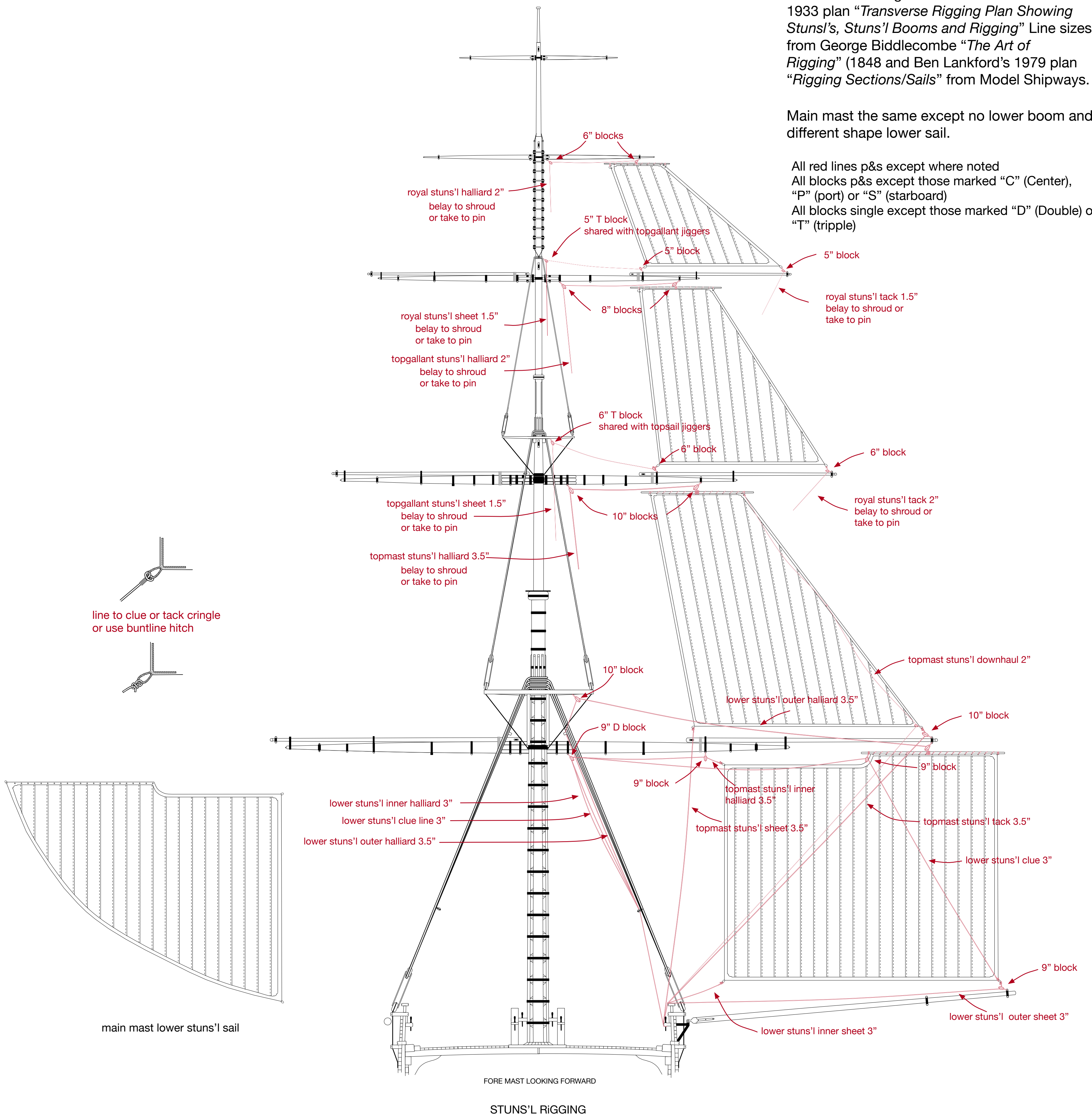
FLYING CLOUD - FORE MAST
