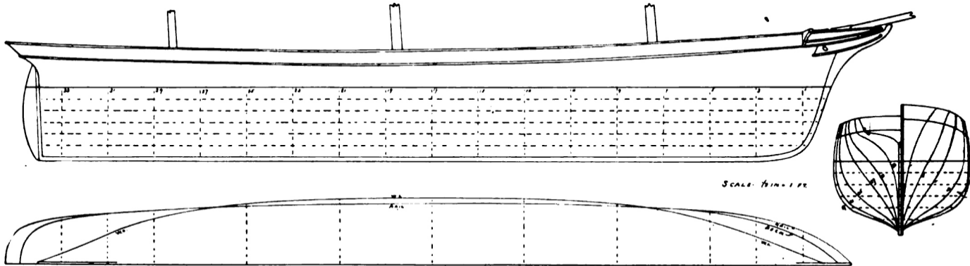
Lines of the Clipper Ship Flying Cloud
