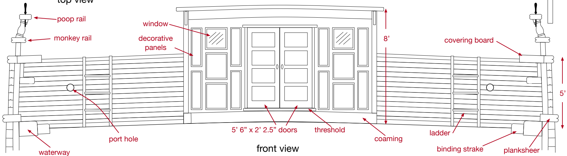
FLYING CLOUD - POOP HOUSE
