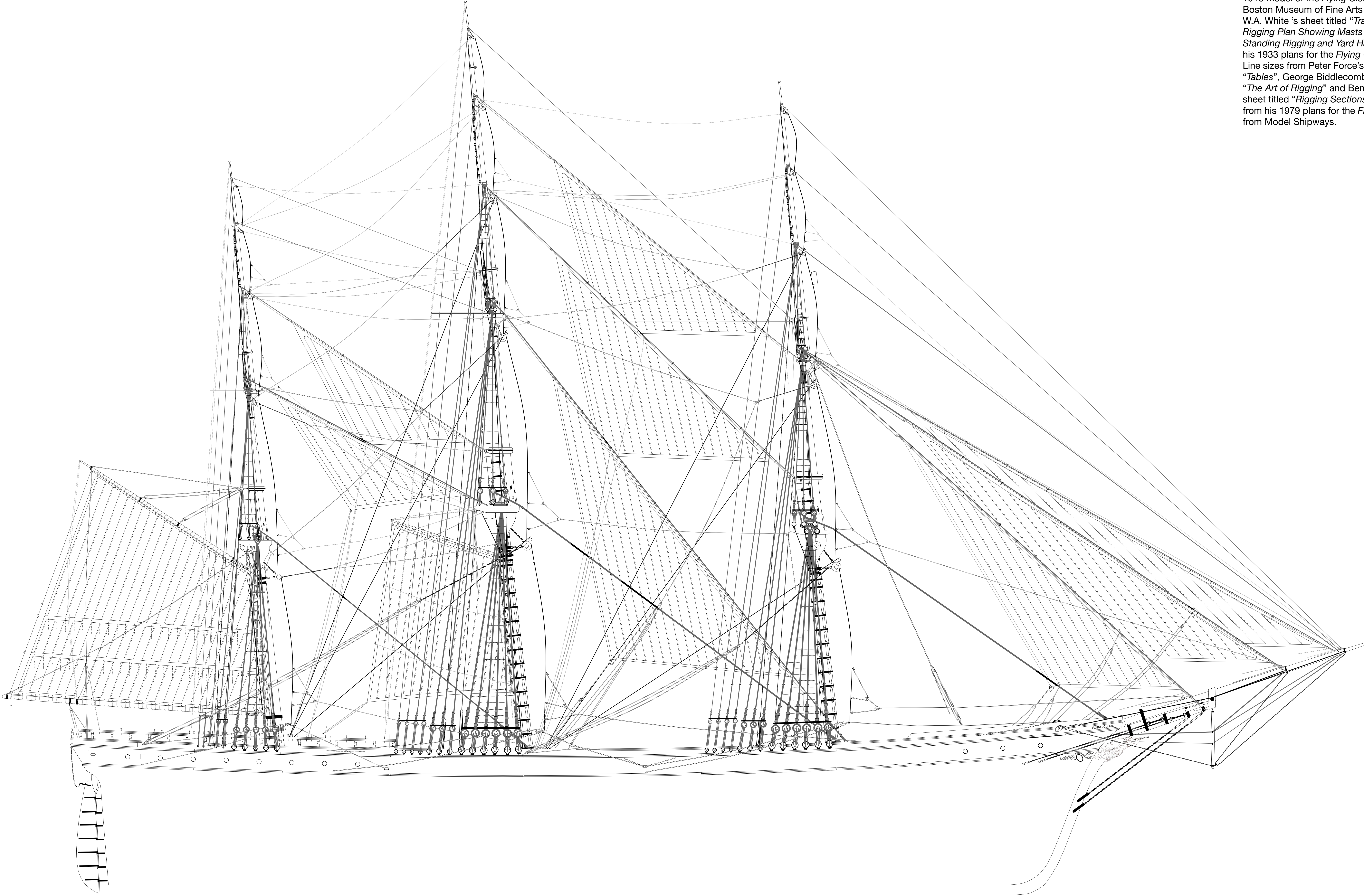
FLYING CLOUD - RIGGING
