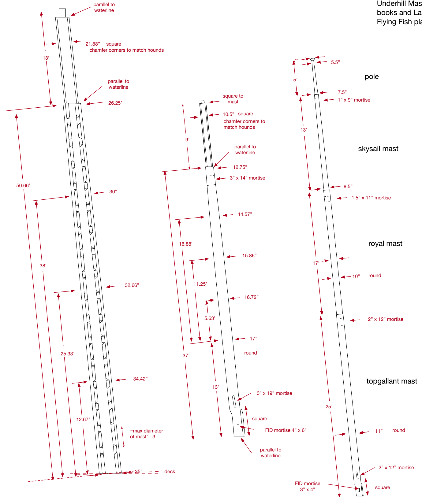
Lower Mast
