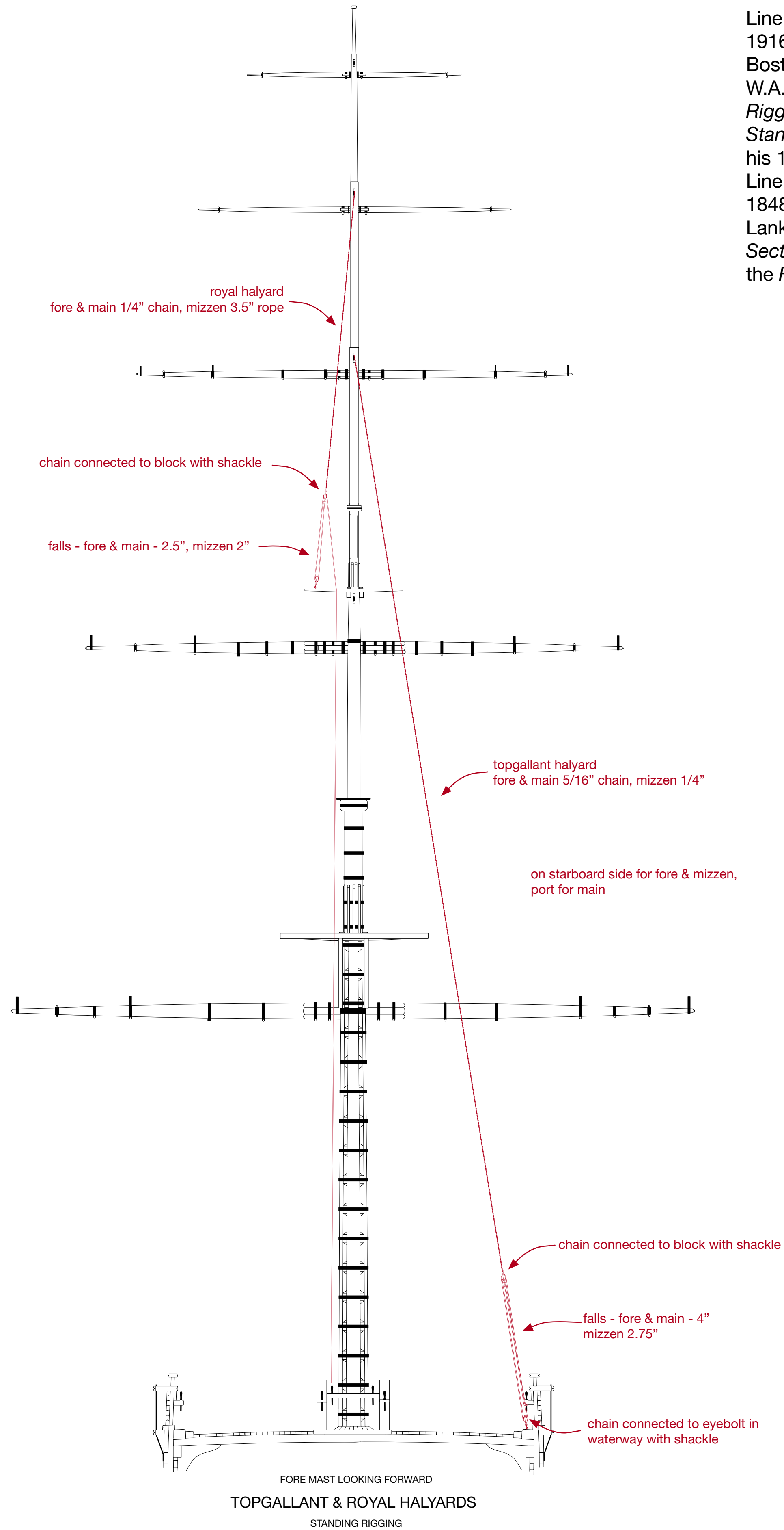
FLYING CLOUD - FORE MAST
