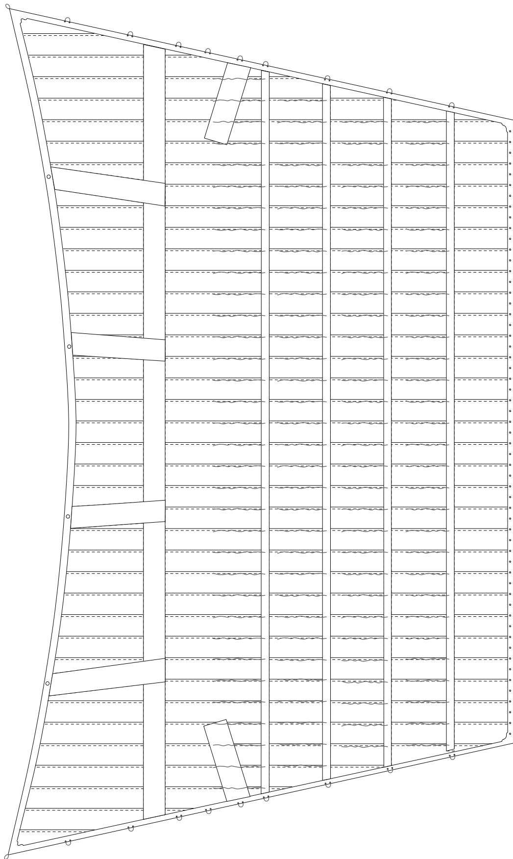
FLYING CLOUD - MAIN TOPSAIL SAIL- FRONT
