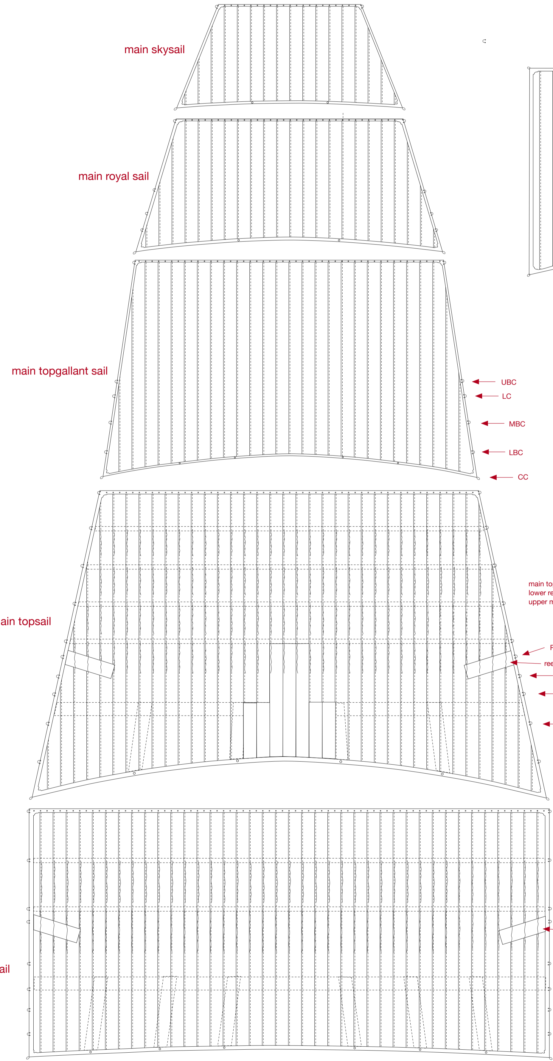
MAIN SAILS
