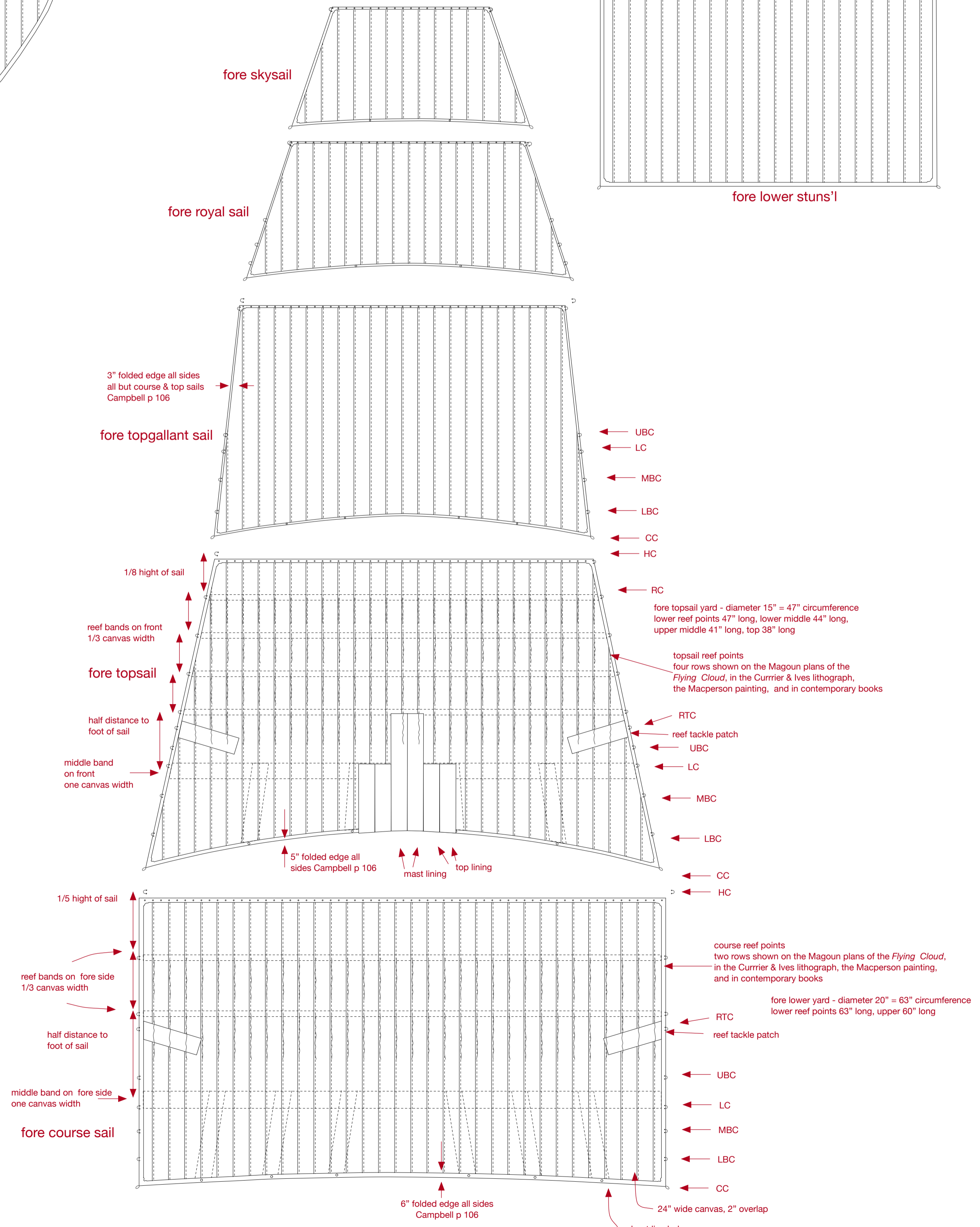
FORE SAILS
