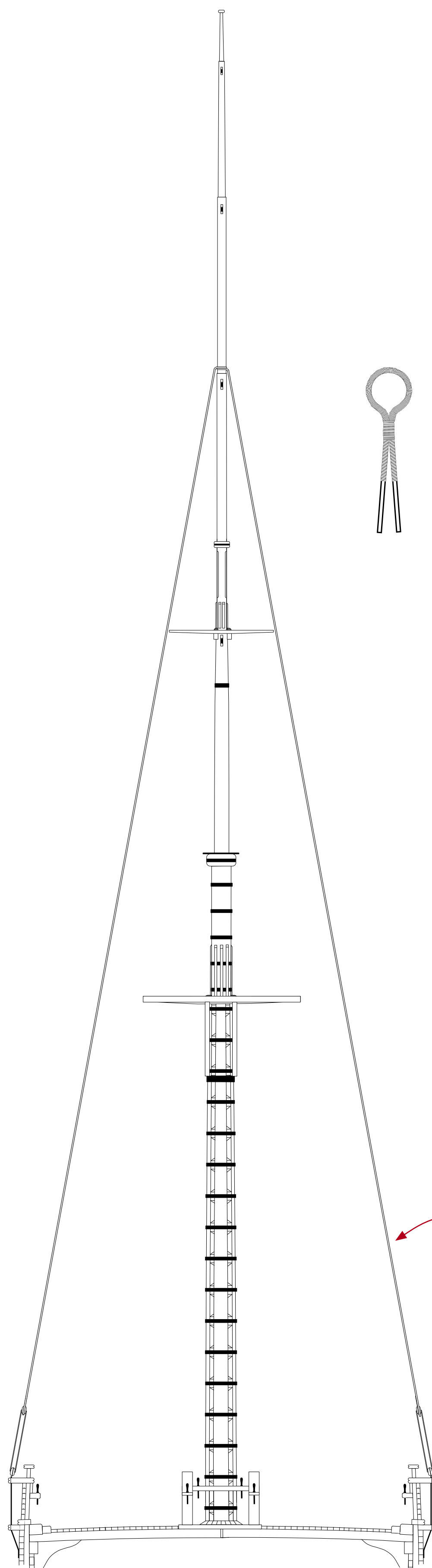
FORE MAST LOOKING FORWARD TOPGALLANT BACKSTAYS STANDING RIGGING
