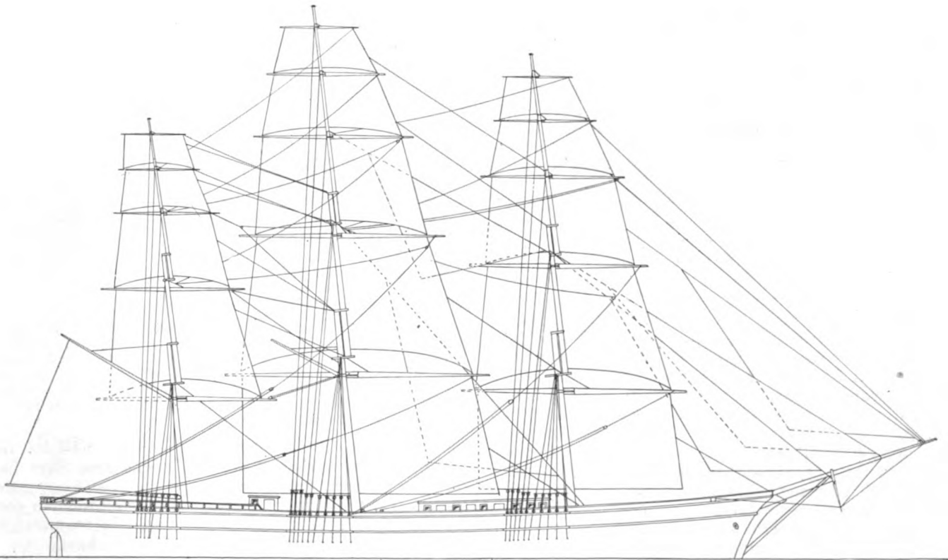
Sail Plan of the Clipper Ship Flying Cloud, Drawn by George B. Douglas
