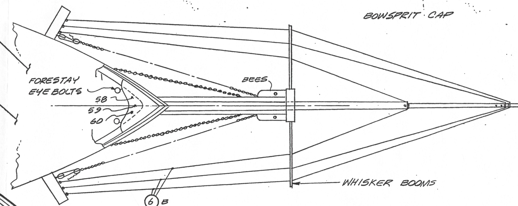
RIGGING OF BOWSPRIT &amp; JIBBOOM
