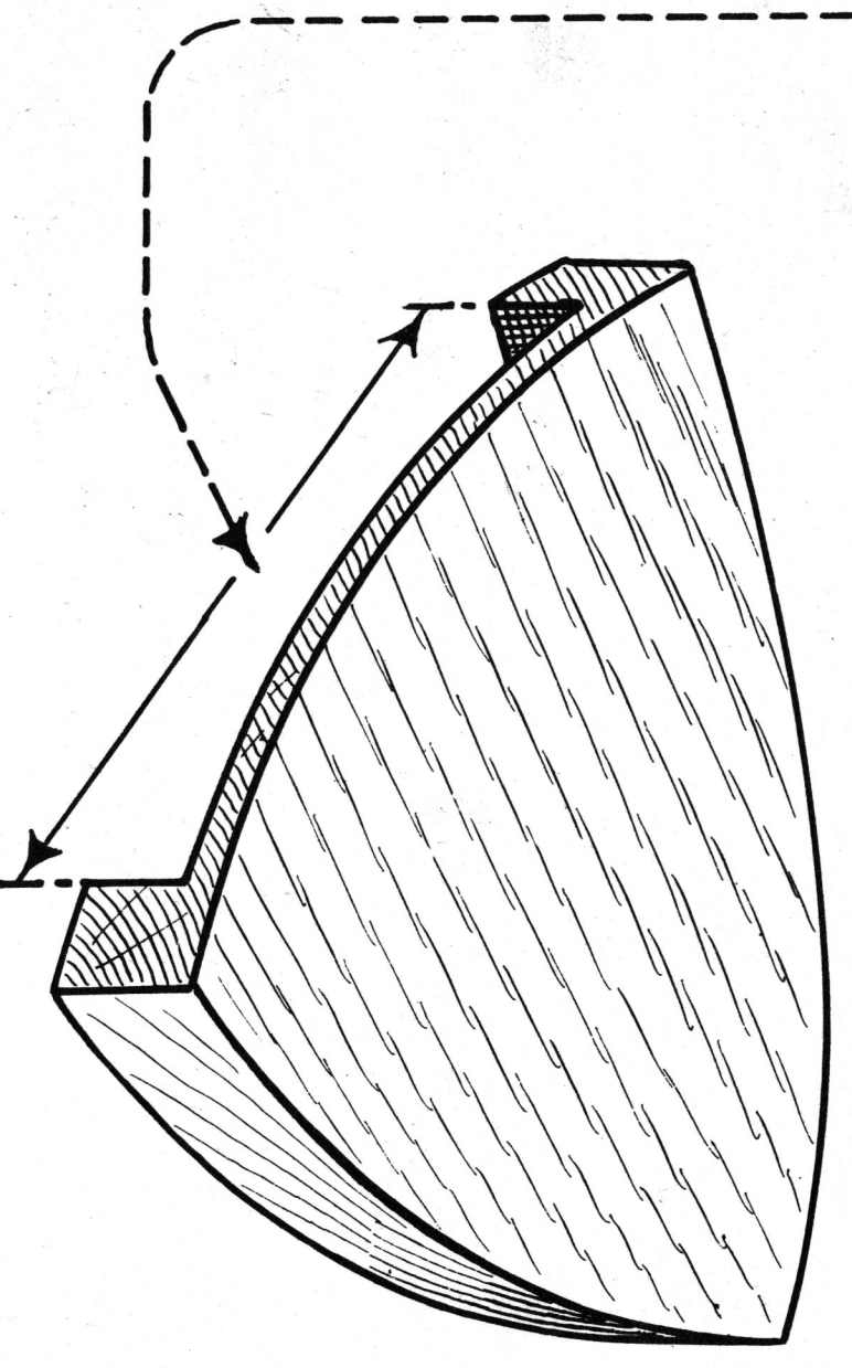
FOC'SLE-HEAD LIFT Fig. 4
