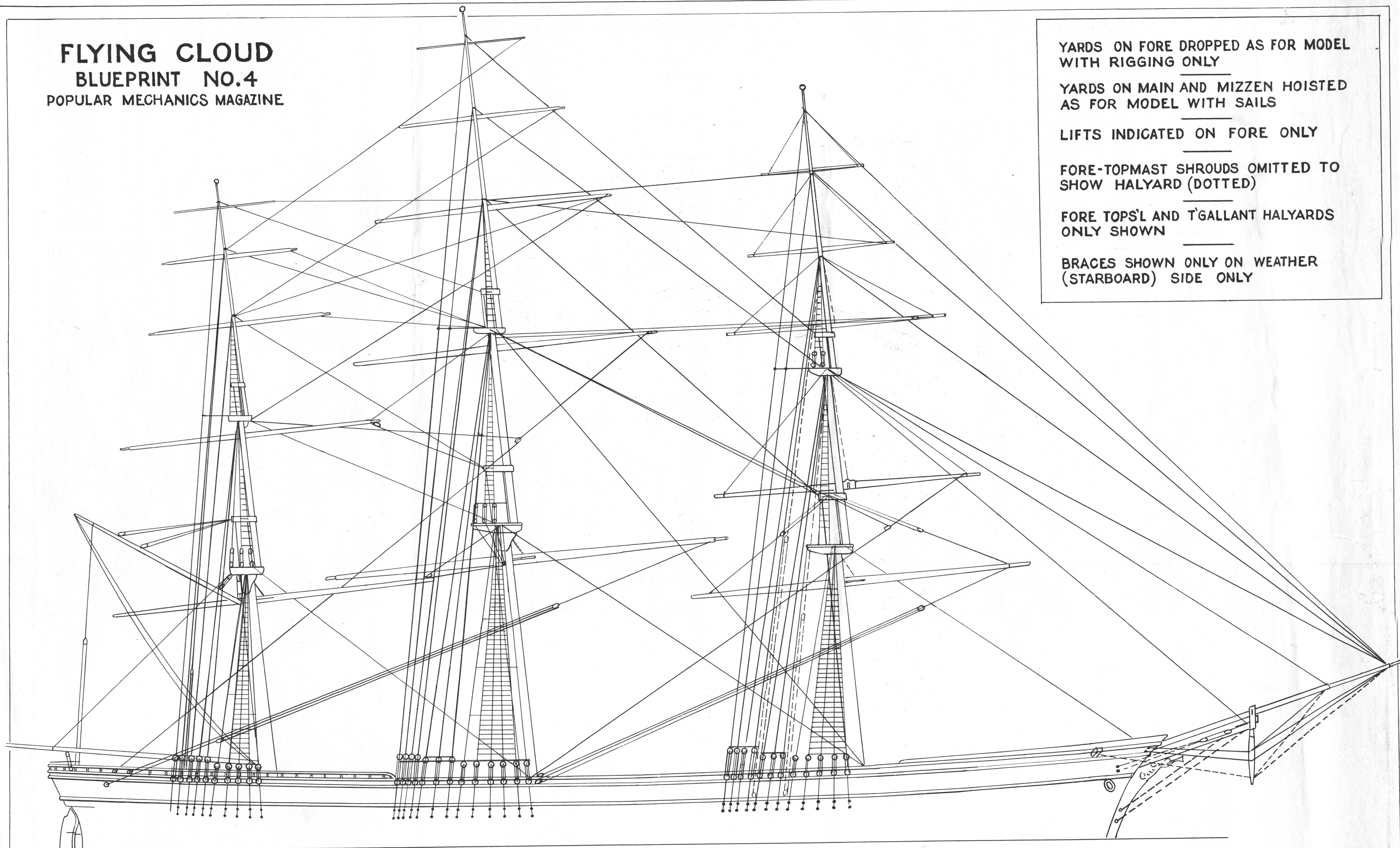
GENERAL RIGGING PLAN
